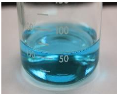
Figure 1. Blue solution of \text{CuCl}_2 \cdot 2\text{H}_2\text{O} .
